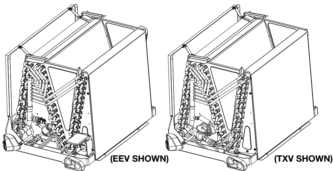
FIGURE 1: DIMENSIONS UNCASSED
